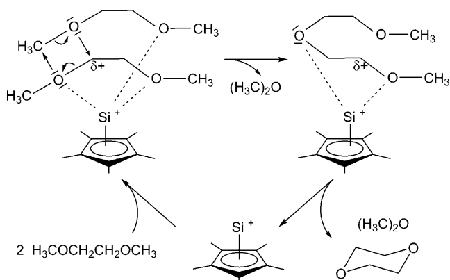
Scheme 2. Suggested catalytic cycle in the transformation of DME into 1,4-dioxane and dimethyl ether. Conceivable weak Si–O interactions are represented by a dotted line.
